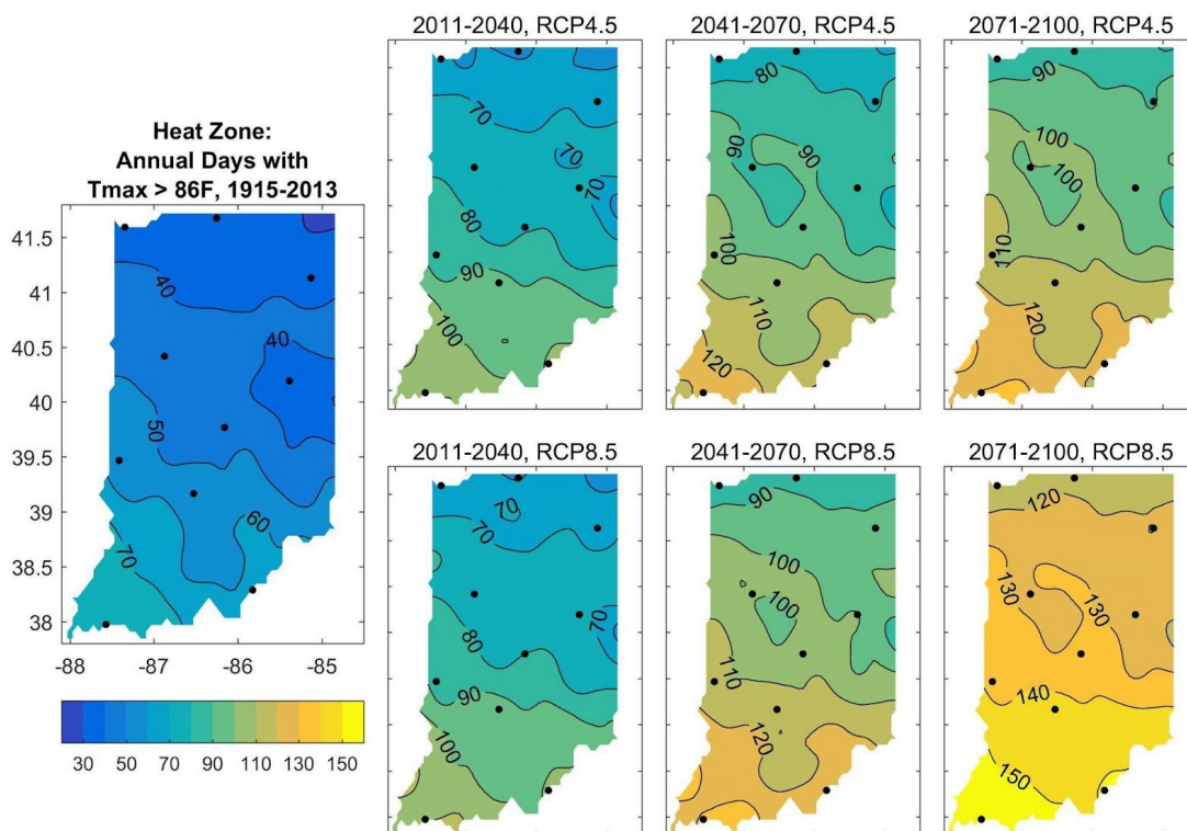
Figure 1. Maps of the historical & projected number of days per year with T_{max} above 86°F for a moderate (top) and very high (bottom) scenario. 9 The axes of the lefthand map denote the latitude (vertical axis) and longitude (horizontal axis).
